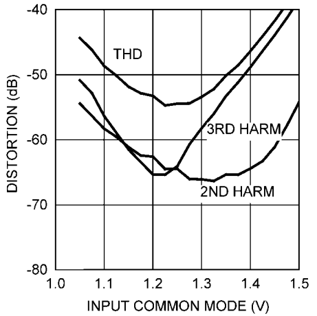
Distortion vs. Input Common Mode
