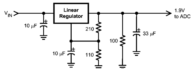
FIGURE 8. Non-Spiking Power Supply
