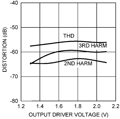
Distortion vs. Output Driver Voltage
