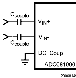
FIGURE 4. Differential Input Drive
