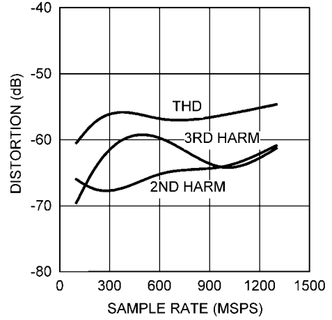
Distortion vs. Sample Rate
