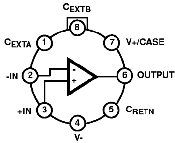
ICL7650S (METAL CAN) TOP VIEW
