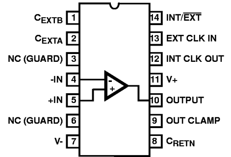
ICL7650S (PDIP, CERDIP) TOP VIEW
