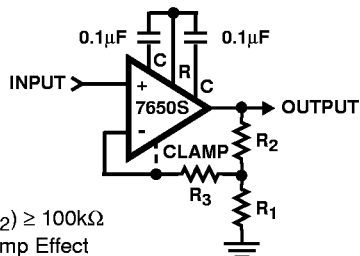
FIGURE 2. NON INVERTING AMPLIFIER WITH OPTIONAL
