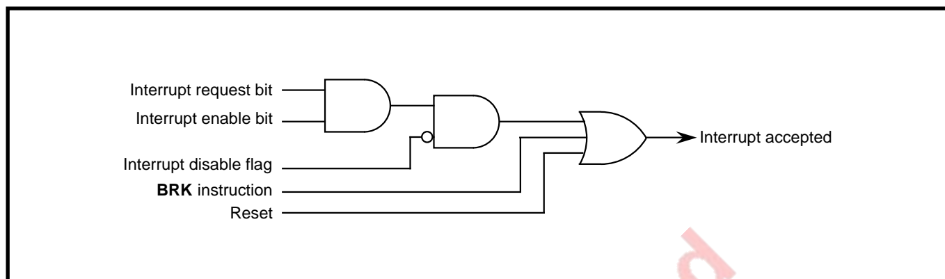
Fig. 1.11.6 Interrupt control diagram
