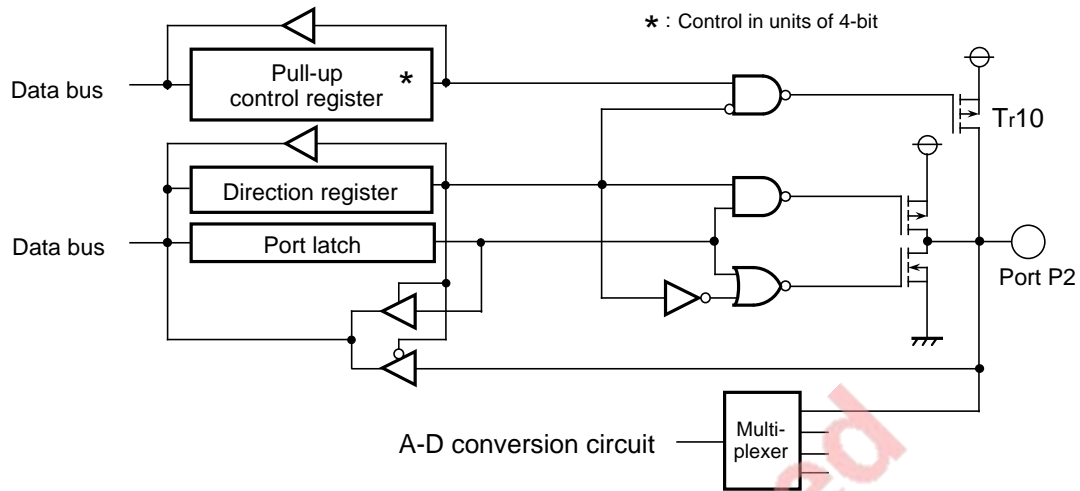
Port P2 (7477/7478 group)
