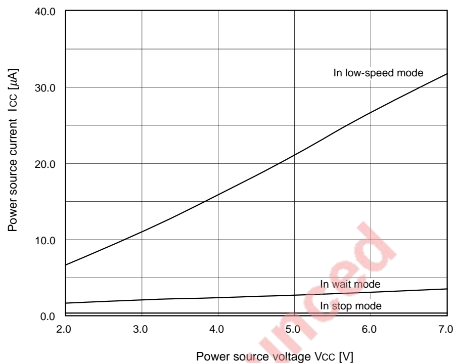
Fig. 1.21.6 I_{CC} - V_{CC} characteristics ( f(X_{CIN}) = 32 \text{ kHz} , 7471 group)
