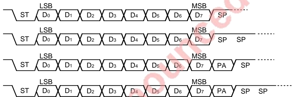
Fig. 1.13B.8 Transmit/receive format of UART
