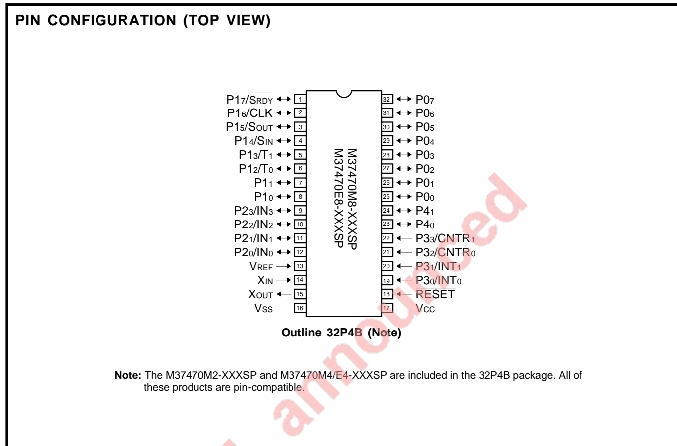
Fig. 1.4.1 Pin configuration of 7470 group
