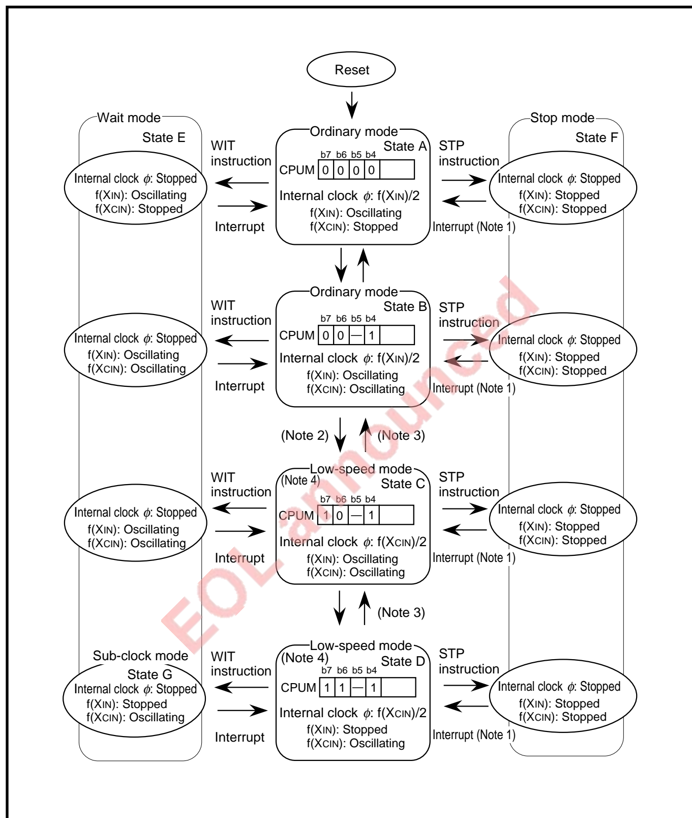
Fig. 1.18.1 State transitions
