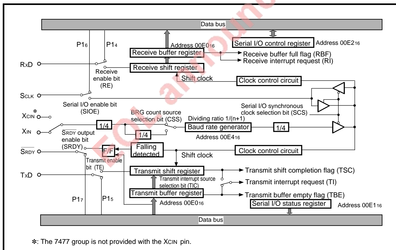
Fig. 1.13B.1 Clock synchronous Serial I/O block diagram
