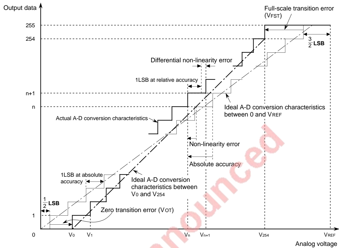
Fig. 1.14.3 Definition of A-D conversion precision
