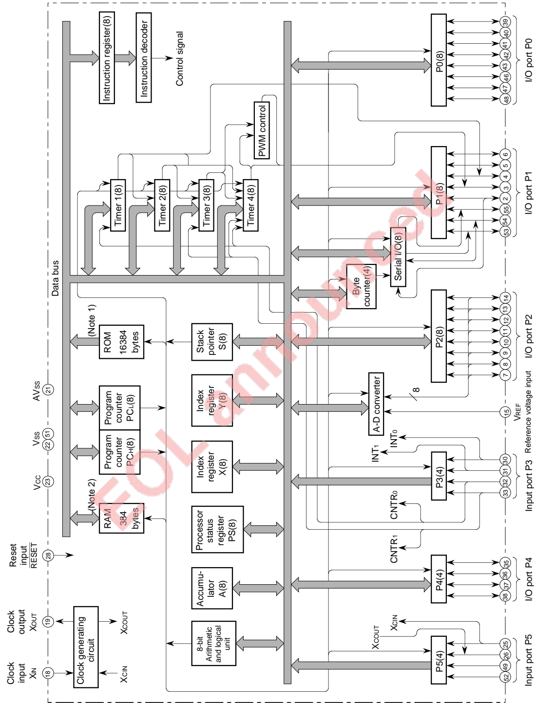
M37471M8/E8-XXXXFP BLOCK DIAGRAM
