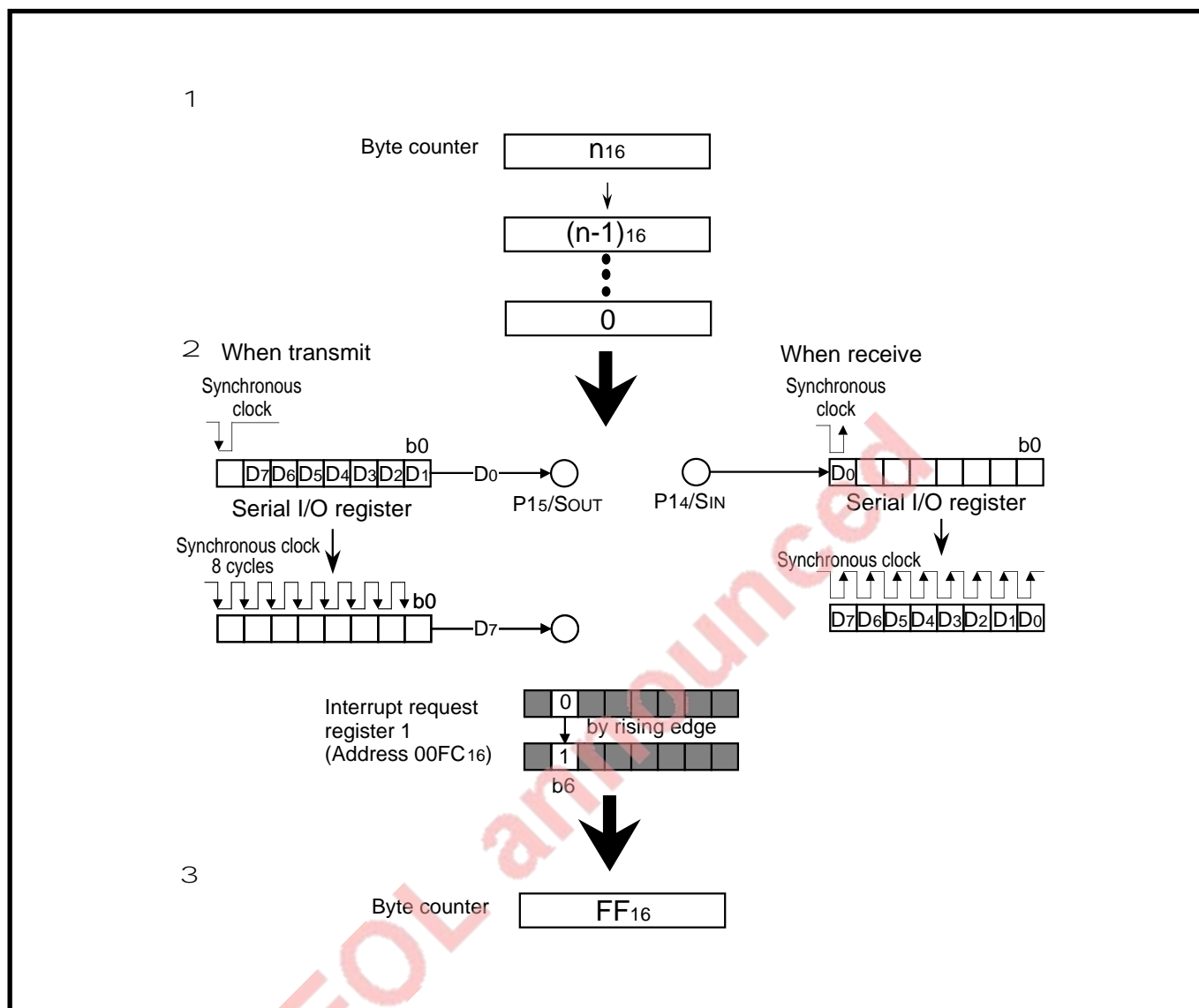
Fig. 1.13A.6 Transmit/receive operation in byte specification mode
