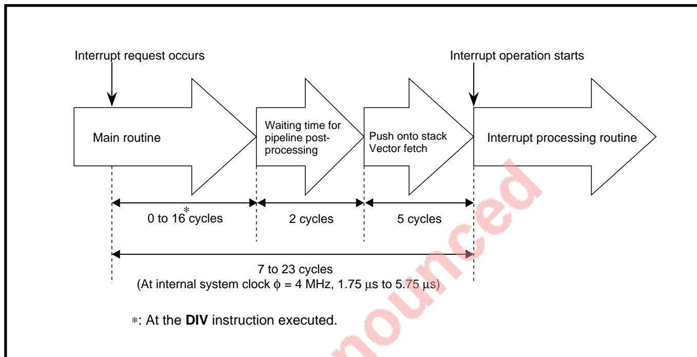
Fig. 1.11.4 Processing time up to the execution of interrupt processing routine
