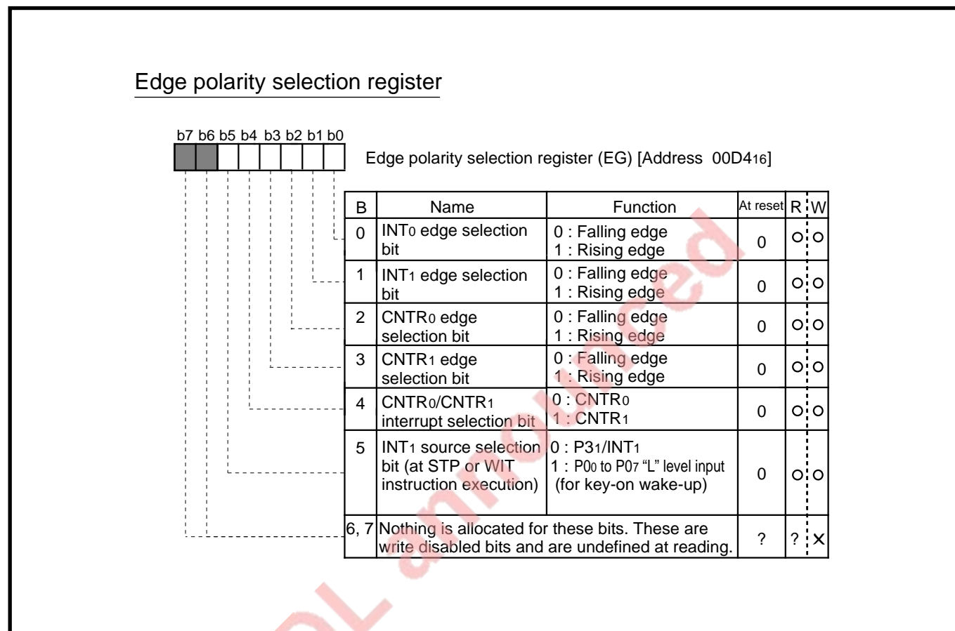
Fig. 1.12.17 Structure of Edge polarity selection register
