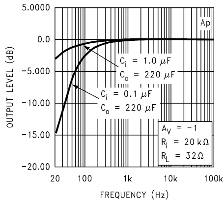
Typical Application Frequency Response
