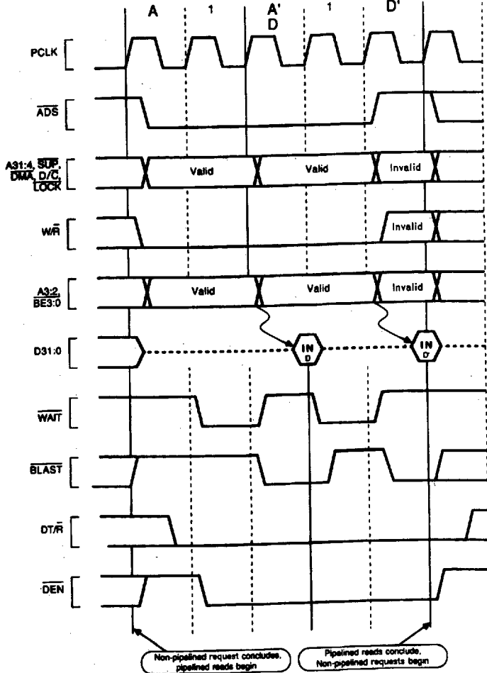
Figure 33. Non-Burst, Pipelined Read Request with Wait States, 32-Bit Bus
