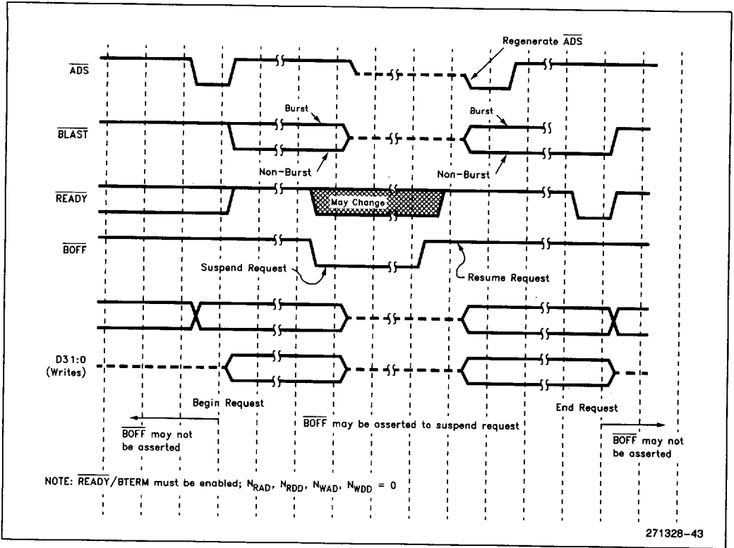
Figure 40. \overline{\text{BOFF}} Functional Timing
