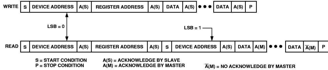
Figure 27. Serial Control Bus—Read and Write Sequences
