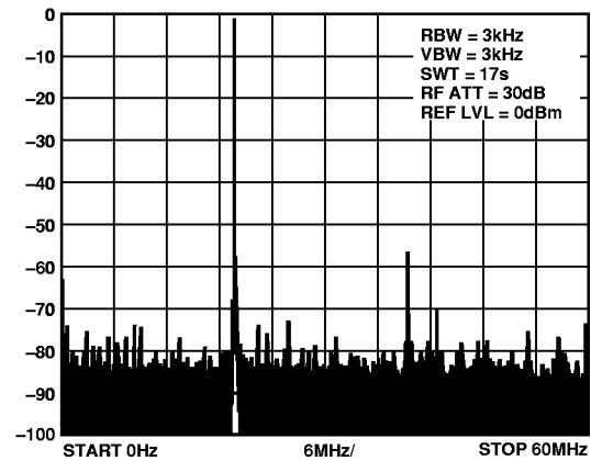
Figure 11. A_{OUT} = 20 MHz
