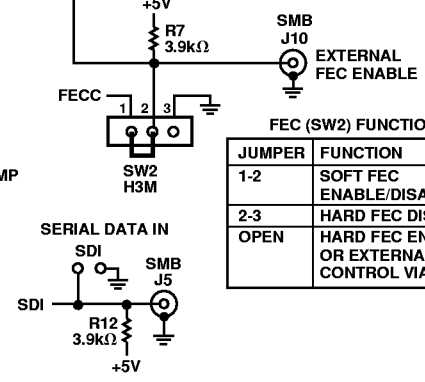
Figure 39. Electrical Schematic of AD9853-xxPCB Evaluation Board
