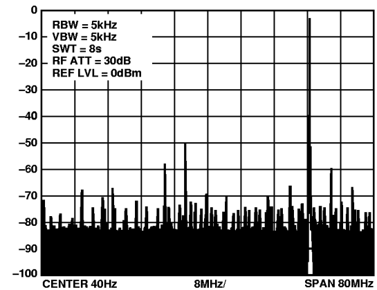
Figure 12. A_{OUT} = 65 MHz (+5 V Supply, 27.5 MHz REFCLK)
