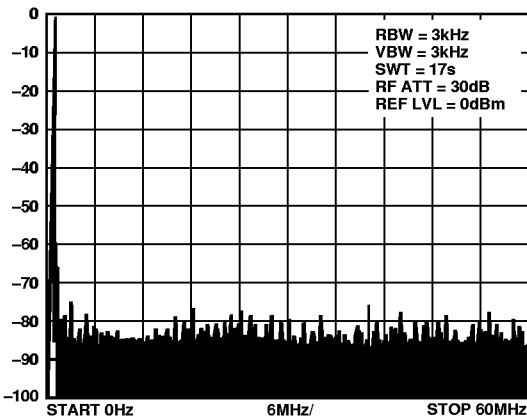
Figure 8. A_{OUT} = 1 MHz
