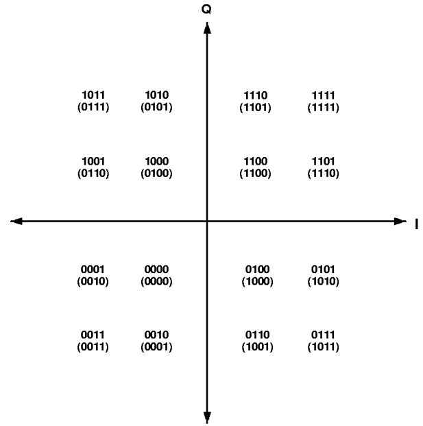
c. 16-QAM Gray-Coded Symbol Mapping
