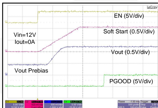
Figure 17. FAN233V06 Startup Waveforms with Pre-Bias Voltage on Output
