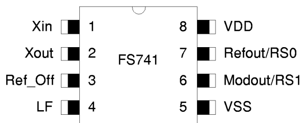
Figure 2. FS741, SOIC Package Pin Assignment
