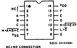
CD4000B
