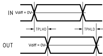
FIGURE 6. Propagation Delay Low-to-High and High-to-Low
