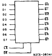
FUNCTIONAL DIAGRAM
