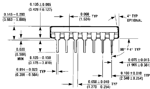
14-Lead Molded Dual-In-Line Package (N) Order Number DM7416N Package Number N14A
