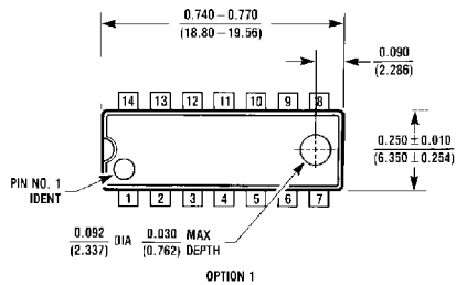
14-Lead Ceramic Dual-In-Line Package (J) Order Number DM5416J Package Number J14A
