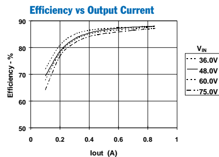
PT4224, V_o = 12.0\text{VDC} (See Note A)
