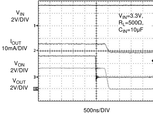
Figure 15. T_{OFF} Response
