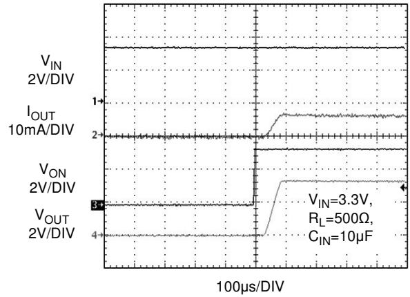
Figure 14. T_{ON} Response
