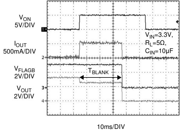
Figure 16. T_{BLANK} Response
