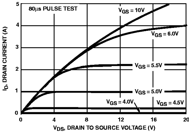
FIGURE 6. SATURATION CHARACTERISTICS
