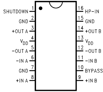
01288128 Top View Order Number LM4863M, LM4863N* See NS Package Number M16B for SO See NS Package Number N16E for DIP*
