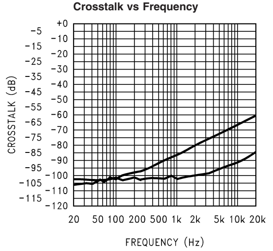
20106135 V_{DD} = 3V ; LLS, RLS; P_O = 200mW ; R_L = 8\Omega ; Mode 7; 0db Gain; 3D off Top-Left to Right; Bot-Right to Left
