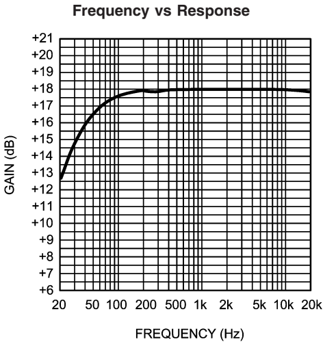
LLS, RLS; R_L = 8\Omega ; Mode 2; Full Gain
