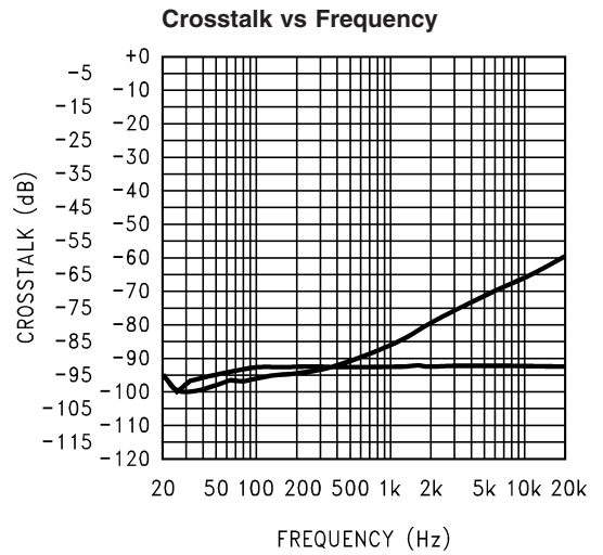
20106137 V_{DD} = 3V ; LHP, RHP; P_O = 10mW ; R_L = 32\Omega ; Mode 9; 0db Gain; 3D off Top-Left to Right; Bot-Right to Left
