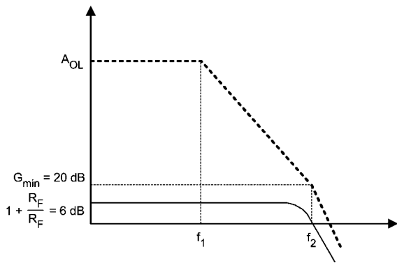
FIGURE 11. Compensation with Reduced Loop Gain
