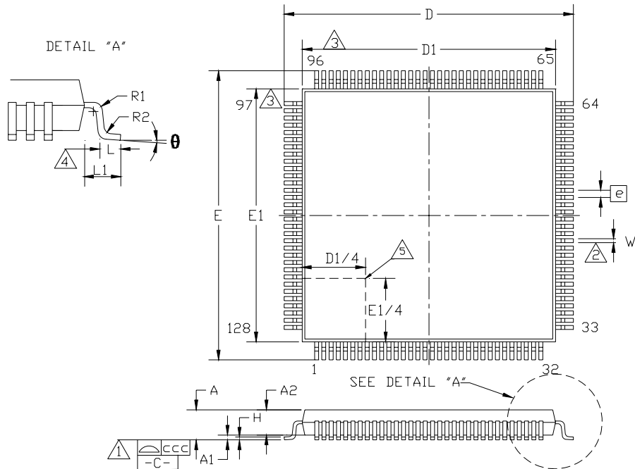
Figure 7.1 USB2227/USB2228 128-Pin VTQFP Package Outline
