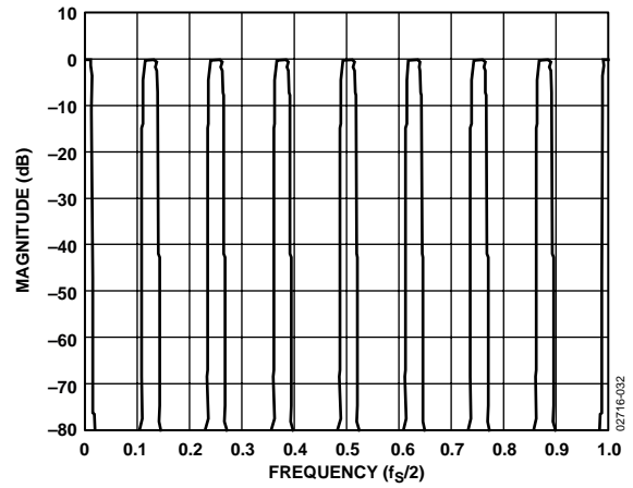
Figure 32. Input Signal Spectrum (N = 4), \alpha = 0.25
