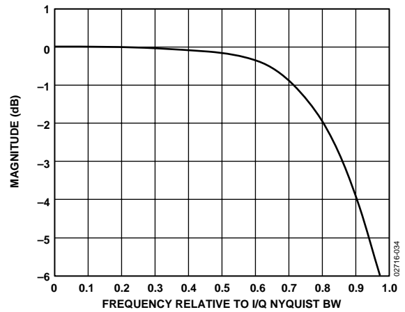
Figure 34. Cascaded Filter Pass-Band Detail (N = 4)
