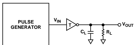
Figure 1. Test Circuit for Driver Propagation Delay and Transition Time
