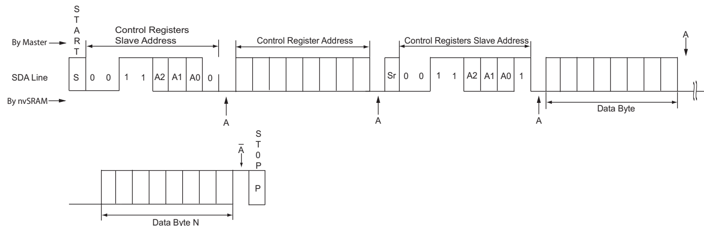
Figure 27. Random Control Registers Multi-Byte Read
