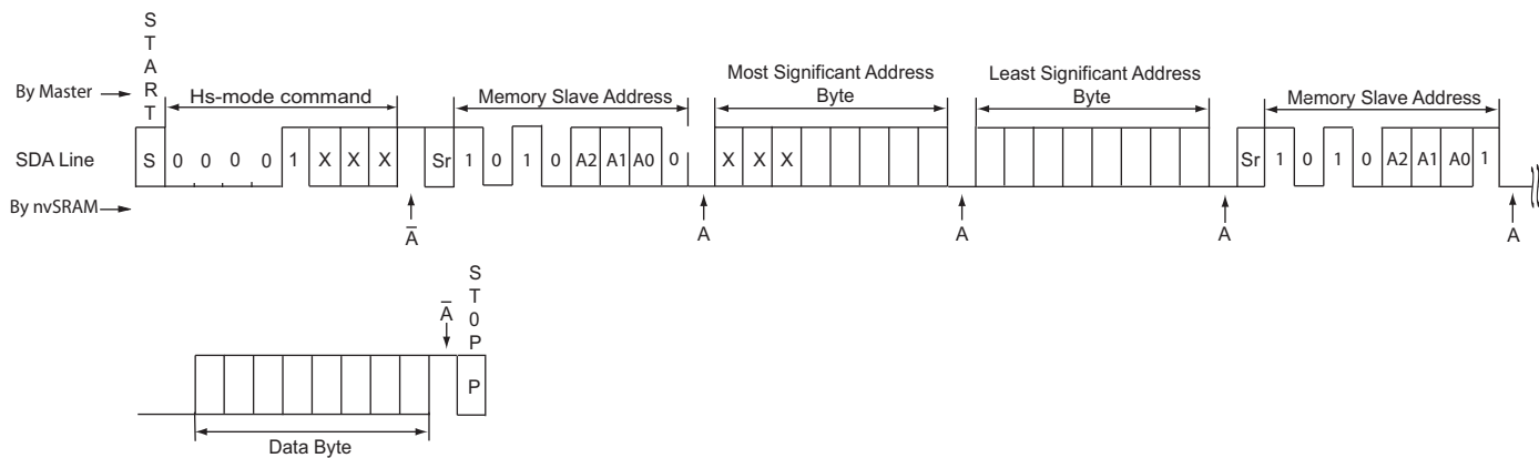
Figure 20. Random Address Single-Byte Read (Hs-mode)
