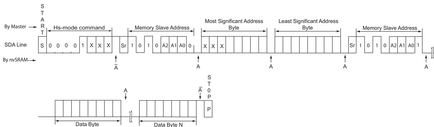
Figure 21. Random Address Multi-Byte Read (Hs-mode)
