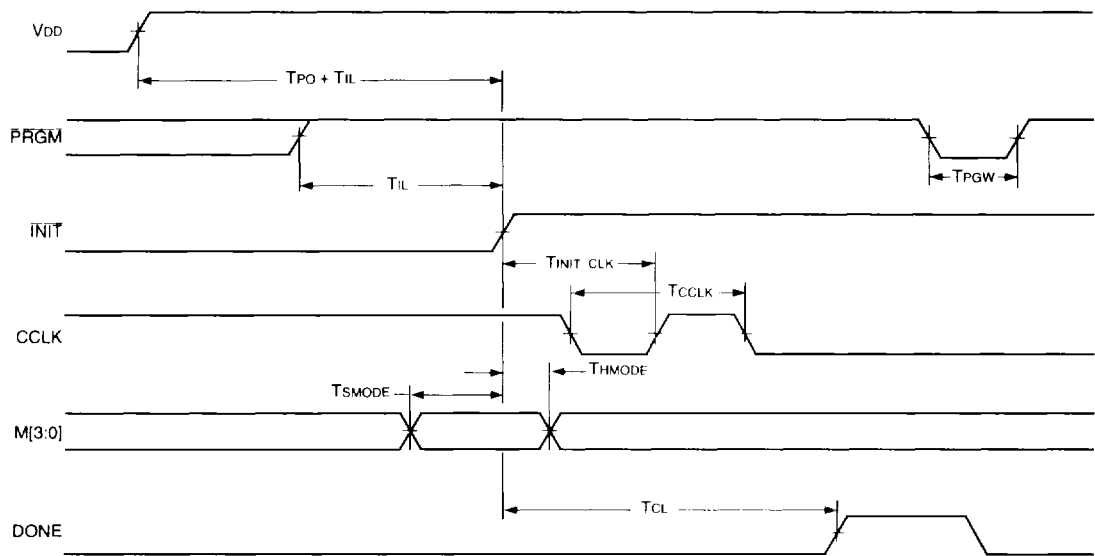
Figure 54. General Configuration Mode Timing Diagram
