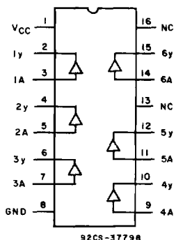
CD54/74HC4050
