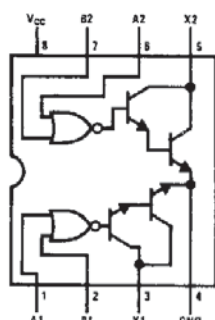
Top View Order Number DS1633J-8 or DS3633N
