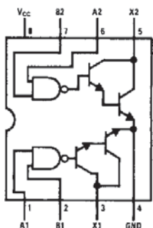
Top View Order Number DS1631J-8 or DS3631N
