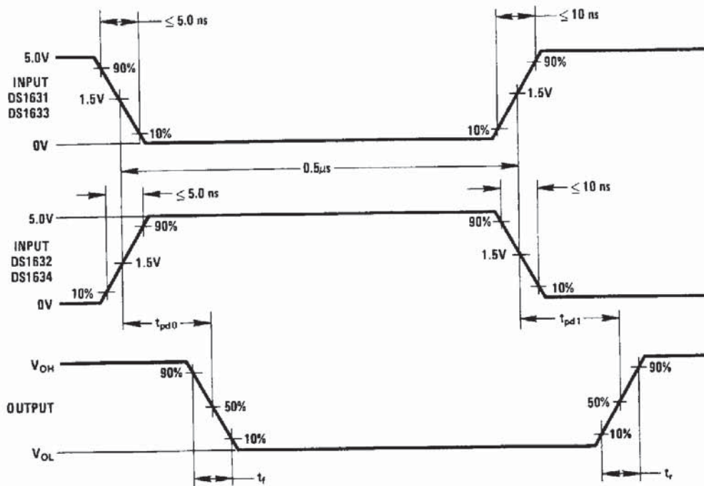
FIGURE 5. Switching Times
