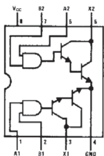
Top View Order Number DS1632J-8 or DS3632N
