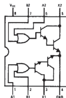
Top View Order Number DS1634J-8 or DS3634N
