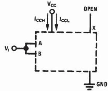
FIGURE 4. I_{CC} for AND and NAND Circuits
