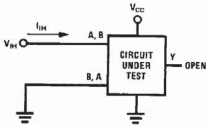
FIGURE 2. I_{IH}
