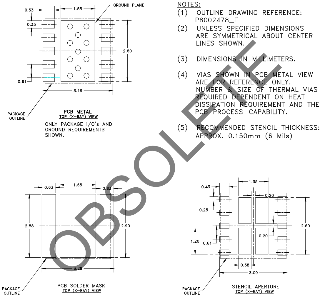
Figure 19: Recommended PCB Layout Information
