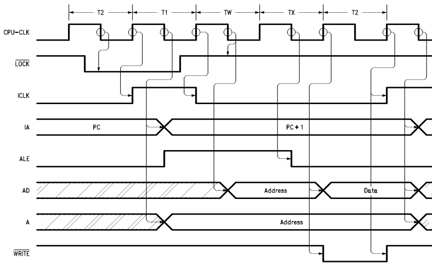
FIGURE 2-30. \overline{\text{LOCK}} Timing
