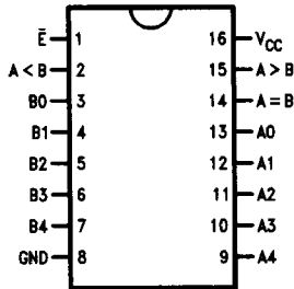
Dual-In-Line Package
