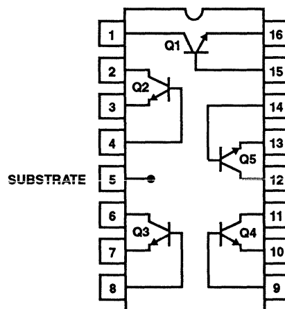
CA3127 (PDIP, CDIP, 150MIL SOIC) TOP VIEW
