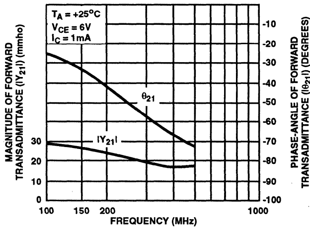
FIGURE 14. FORWARD TRANSMITTANCE ( Y_{21} ) vs FREQUENCY
