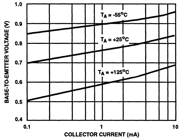
FIGURE 4. BASE-TO-EMITTER VOLTAGE vs COLLECTOR CURRENT
