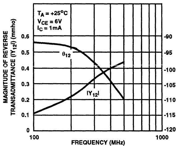
FIGURE 16. REVERSE TRANSMITTANCE ( Y_{12} ) vs FREQUENCY
