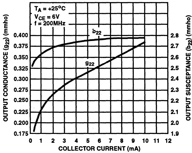
FIGURE 12. OUTPUT ADMITTANCE ( Y_{22} ) vs COLLECTOR CURRENT
