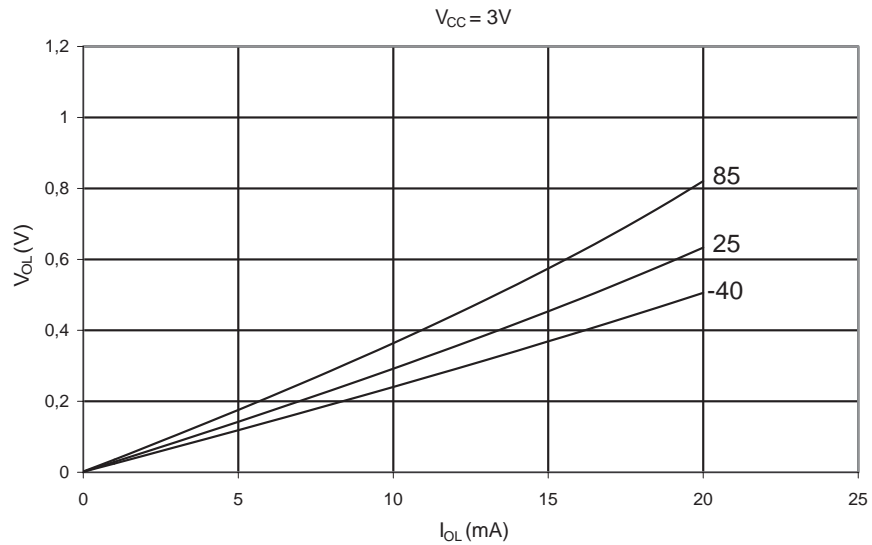
Figure 25-19. I/O Pin Output Voltage vs. Sink Current ( V_{CC} = 3V )
