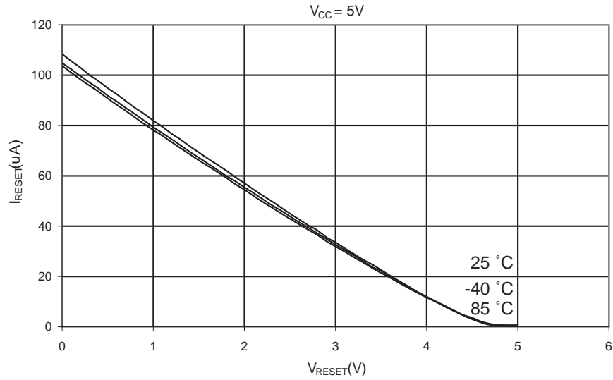
Figure 25-18. Reset Pull-up Resistor Current vs. Reset Pin Voltage ( V_{CC} = 5V )
