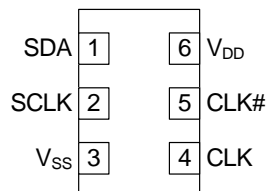
Figure 1. 6-pin Ceramic LCC pinout
