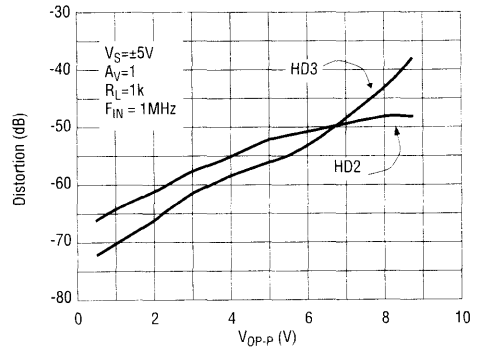
Harmonic Distortion vs V OP-P
