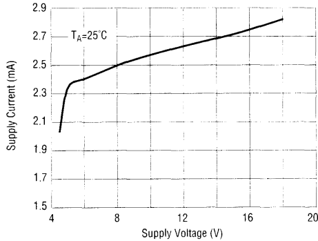
EL5410C Supply Current per Amplifier vs Supply Voltage
