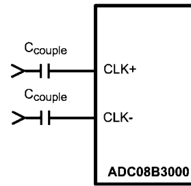
FIGURE 20. Differential Sample Clock Connection
