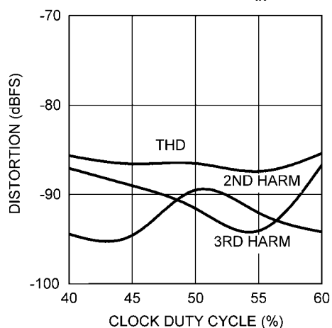
Distortion vs. Clock Duty Cycle, f_{IN}=40\text{ MHz}
