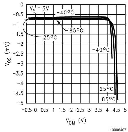
Offset Voltage vs. Common Mode Voltage ( V_S = 5V )
