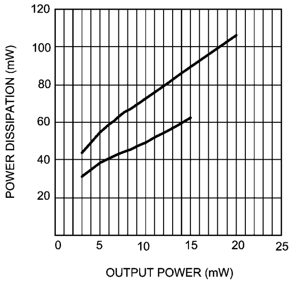
Power Dissipation vs Output Power V_{DD} = 1.8V , f = 1kHz , from top to bottom: R_L = 16\Omega ; R_L = 32\Omega
