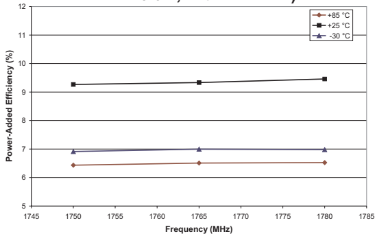
Figure 14: Power-Added Efficiency vs. Freq. ( P_{OUT} = +16.0 dBm, V_{CC} = +3.5 V, V_{REF} = +3.0 V, V_{MODE} = +2.7 V)
