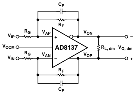
Figure 63. Typical Connection
