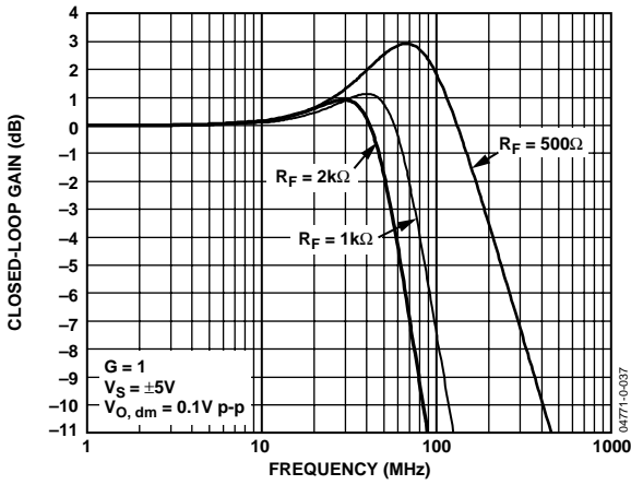
Figure 19. Small Signal Frequency Response for Various R_f
