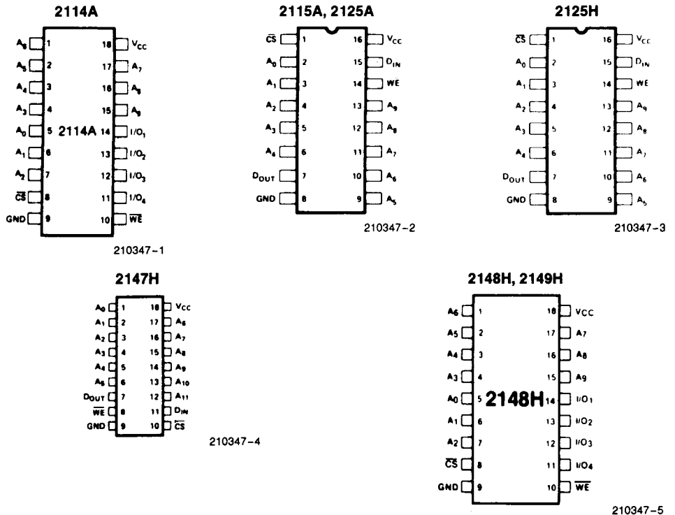
Pin Configuration
