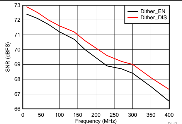
f_S = 160\text{ MSPS} , f_{IN} = 100\text{ MHz}
