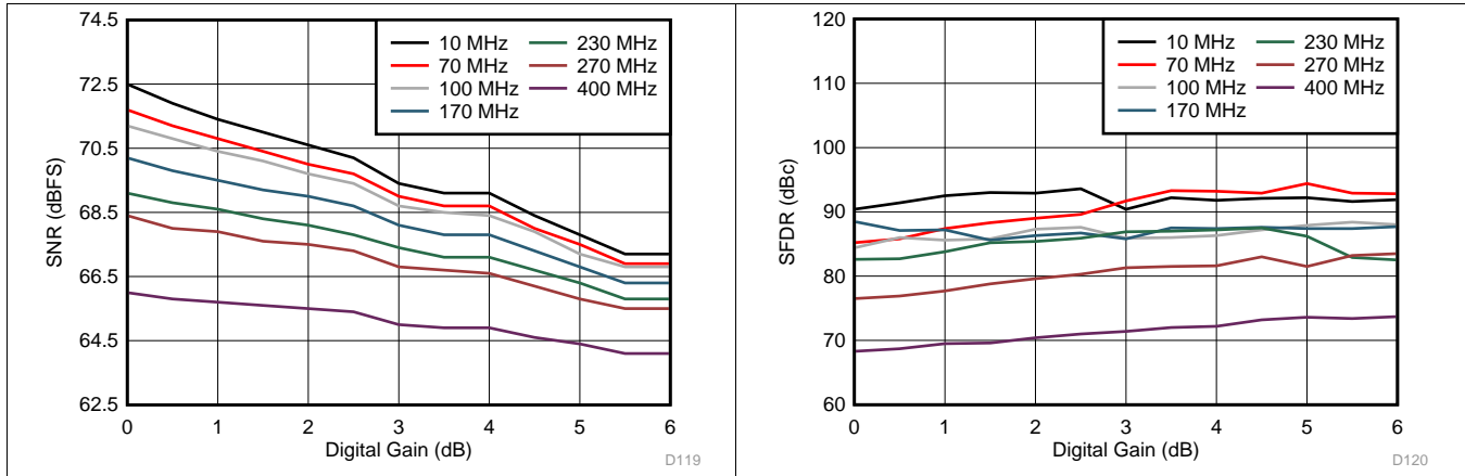
Figure 19. Signal-to-Noise Ratio vs Digital Gain and Input Frequency
