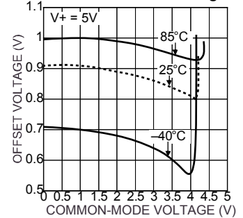
Offset Voltage vs. Common-Mode Voltage
