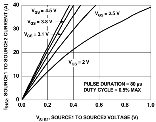
Figure 2. On-Region Characteristics
