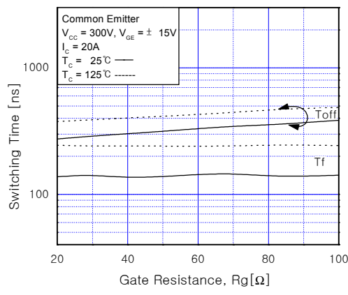
Fig 8. Turn-Off Characteristics vs. Gate Resistance
