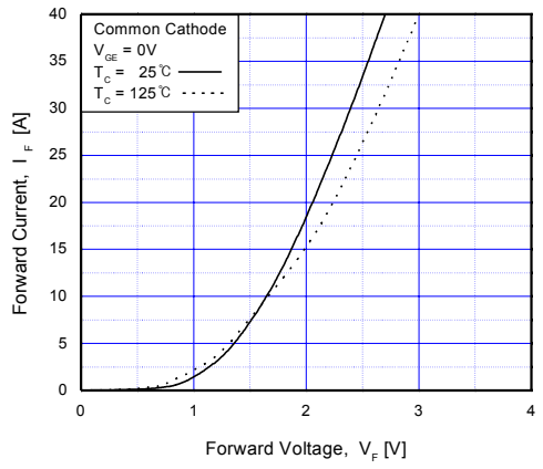
Fig 15. Forward Characteristics
