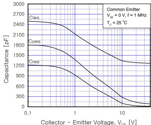
Fig 6. Capacitance Characteristics
