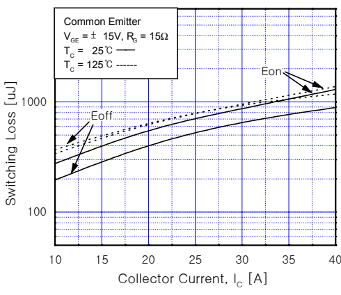
Fig 12. Switching Loss vs. Collector Current
