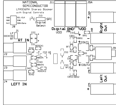
Silk Screen
