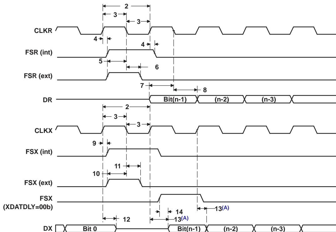
Figure 5-48. McBSP Timing
