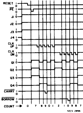
Fig. 3 – CD40192B timing diagram.
