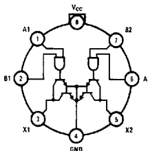
Top View Order Number DS1632J-8 or DS3632N See NS Package Number J08A or N08E
