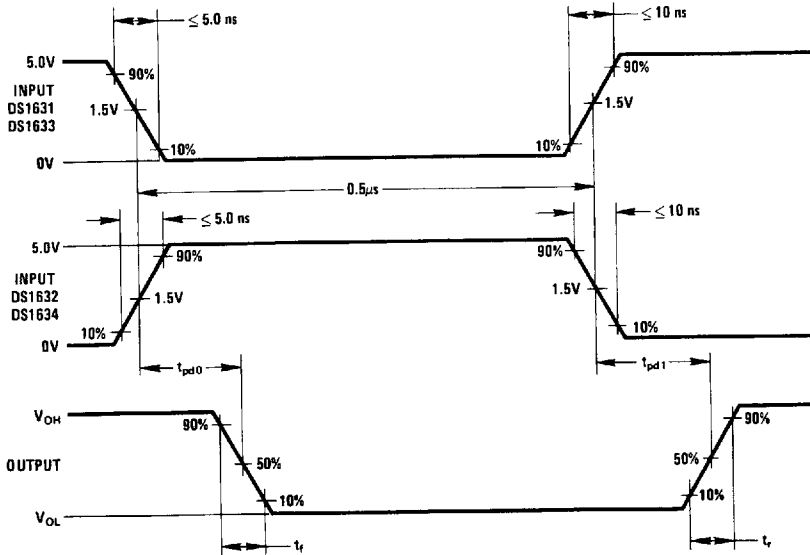
FIGURE 5. Switching Times
