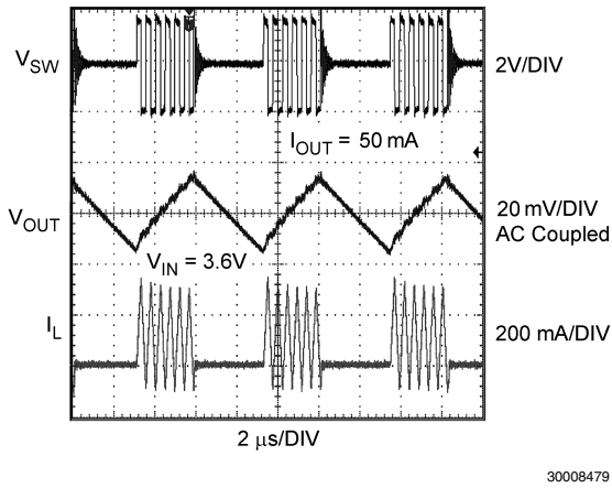
FIGURE 7. Typical PFM Operation
