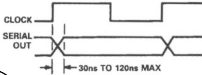
Figure 10. Clock High to Serial Out Valid
