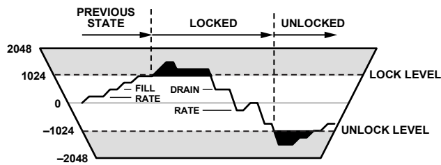
Figure 41. Lock Detector Diagram
