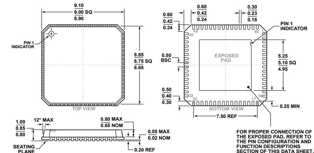
Figure 61. 64-Lead Lead Frame Chip Scale Package [LFCSP_VQ]
